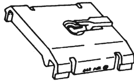
89-6674 Replaces: 20474691 CLIP-BODY SIDE MOULDING DOOR QUARTER PANEL Plastic G.M. "W" Body '88/ UNIT PACKAGE 25
