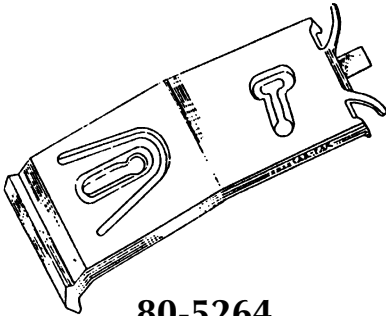
80-5264 Replaces: 6003777 CLIP-SILL MOULDING Chrysler Products '81/ UNIT PACKAGE 25
