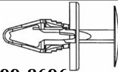
99-8696 Replaces: 11589289, W713610-S300, 6508863AA RIVET-DRIVE TYPE, Flares, Cowl, RKR Moulding,, Front Bumper, Plastic Hole: M6.25-6.53, Flange: 18MM, Stem Lgth: 17.5MM, P.R.: 2-4MM G.M. Equinox & Torrent 2007, Buick Enclave, Saturn '91/, Ford Focus 2008/ & Dodge PU 2009/ UNIT PACKAGE 25
