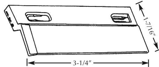
87-6363 Replaces: 20641049 & 10091281 CLIP-ROCKER PANEL MOULDING L.H. Plastic Accent Moulding Pontiac Grand Prix '88/ UNIT PACKAGE 15
