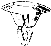
79-5108 Replaces: 800737-S PIN-PUSH TYPE Plastic Hole: M6.3, Head: 22MM, O/L: 17MM Ford Products UNIT PACKAGE 100
