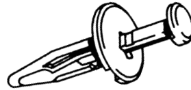
93-7145 Replaces: 10134407, 15990756, F50C-9E728-AA, 6501925 RIVET-DRIVE TYPE, BUMPER, ROCKER MOULDING Hole: M6.3, Flange: 17MM P.R.: 1.52MM - 7.62MM Chrysler "LH" '93/, Dodge Nitro 2007/, Jeep Liberty 2002, Dodge Journey 2009 Ford & G.M., Hummer H2 UNIT PACKAGE 25
