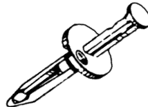
85-5945 Replaces: N803709-S, 15681408, 4857108 RIVET-DRIVE TYPE, BUMPER, FASCIA & FENDER APRON Hole: M6.3, P.R.: 5 - 10MM, Flange: 15MM Plastic Ford '86/, G.M., Chrysler '97/ & Jeep 2005/ UNIT PACKAGE 50
